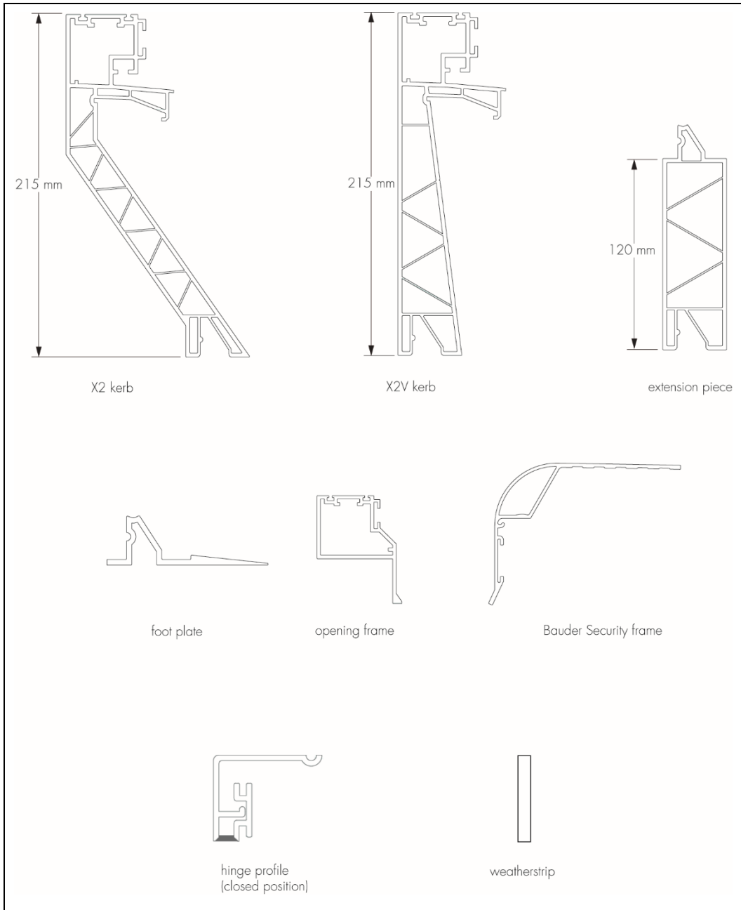
Figure 1 Bauder Euroglaze components
