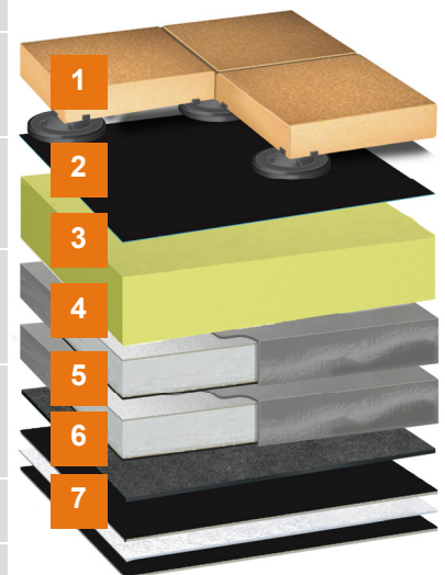
Build-up to achieve 0.16 on a concrete deck
