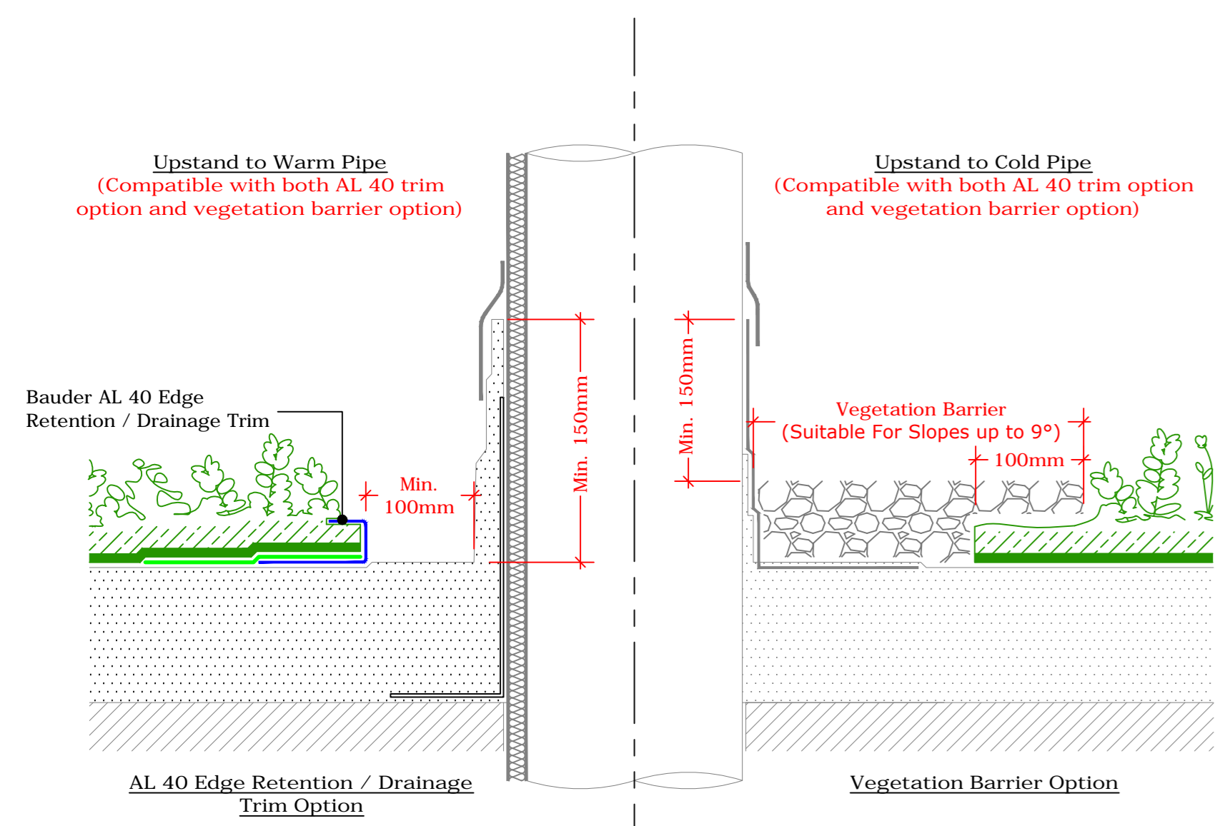
Upstand to Hot Flue or Cold Pipe (Drg.No: D0901-00W_3Deg+_307-Ext-XF301_002)
