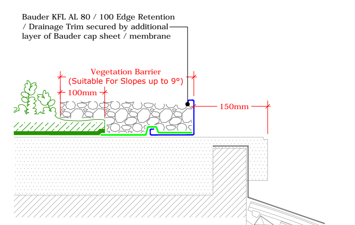
Detail to Mansard Roof (Drg.No: D0901-00W_3Deg+_006-Ext-XF301_006)
