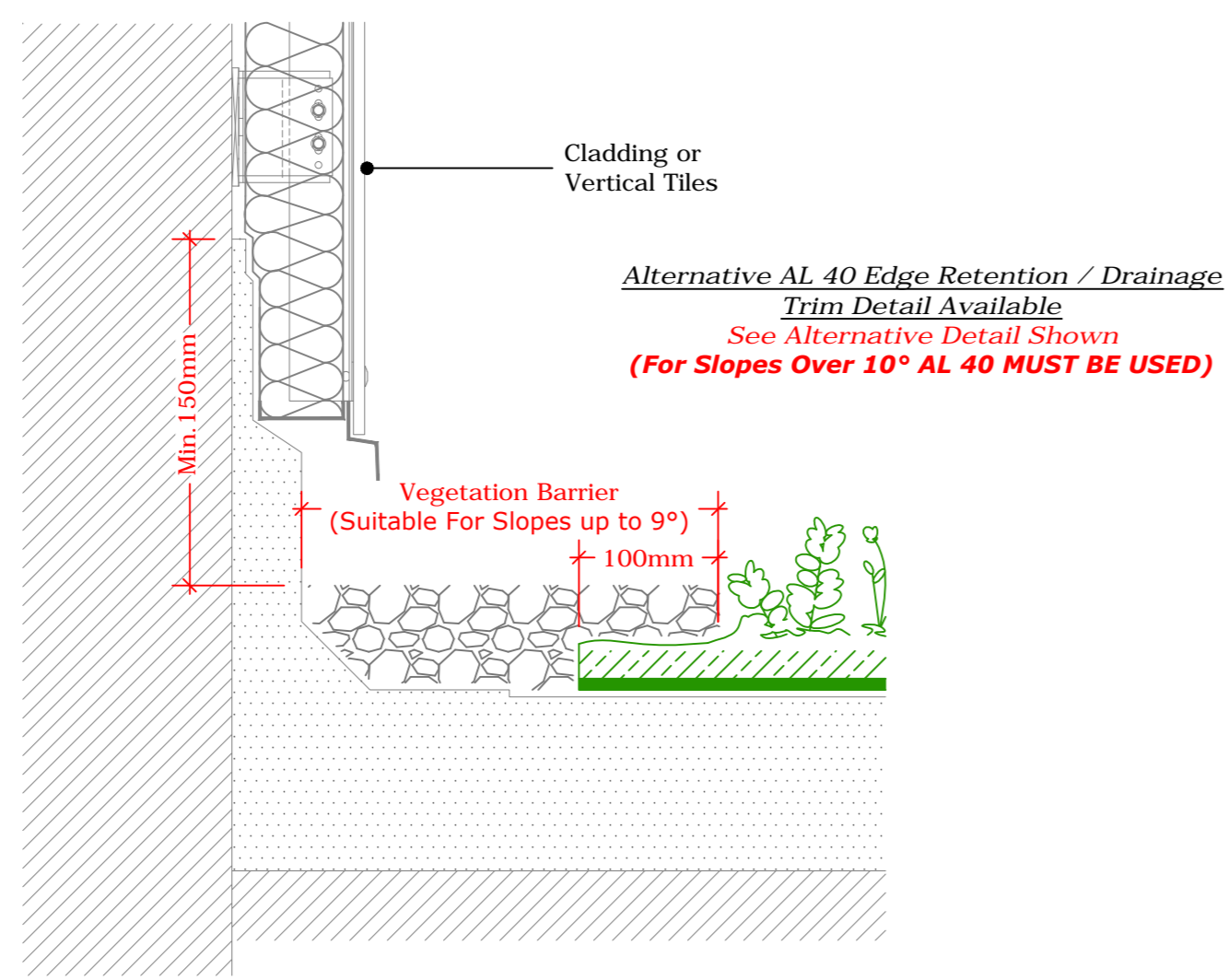
Upstand to Vertical Cladding or Slates/Tiles (Drg.No: D0901-00W_3Deg+_201-Ext-XF301_002)
