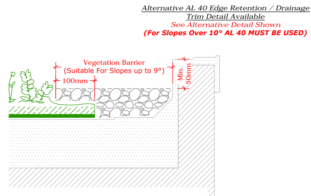
Perimeter Kerb (Drg.No: D0901-00W_3Deg+_002-Ext-XF301_001)
