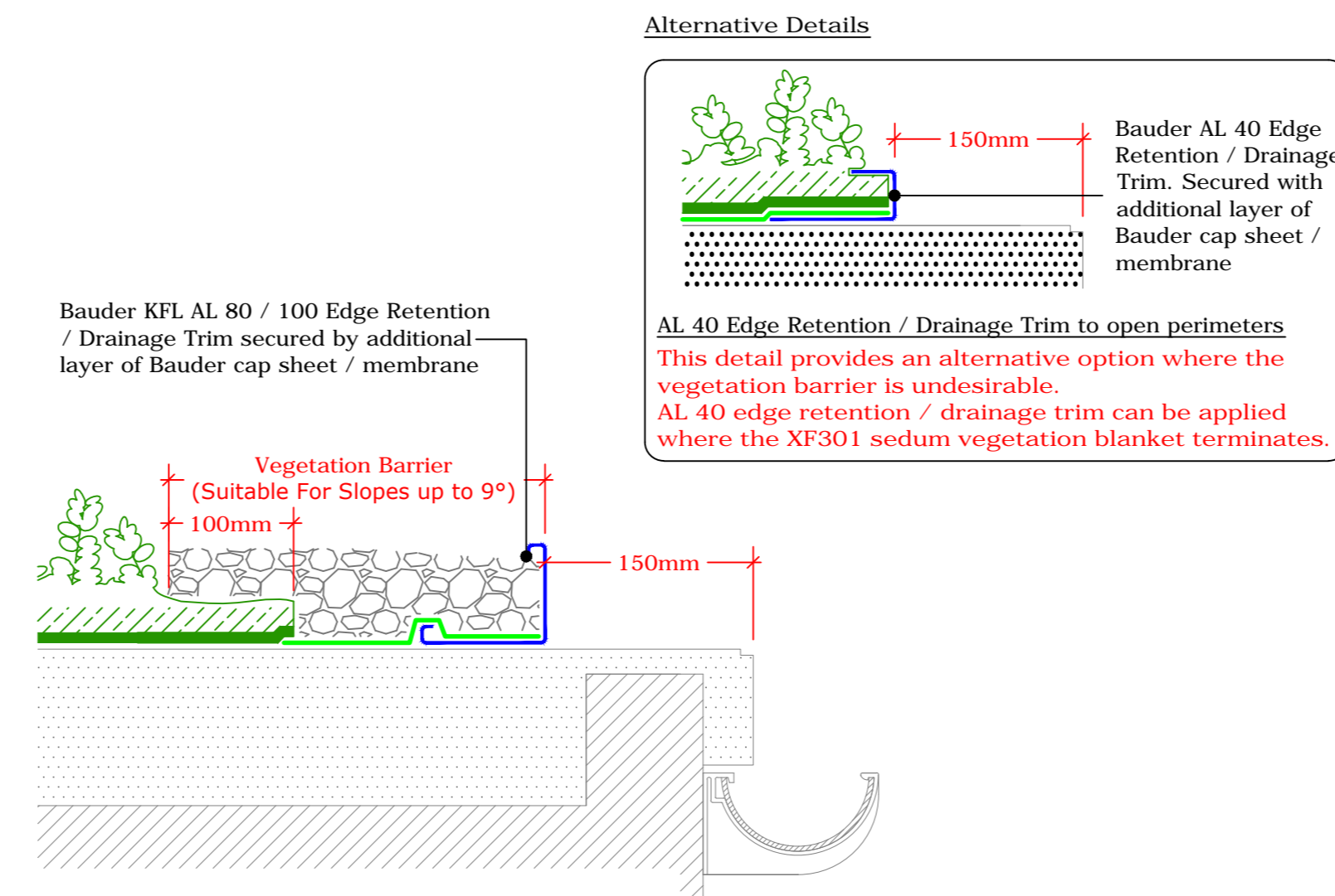
External Gutter (Drg.No: D0901-00W_3Deg+_006-Ext-XF301_005)
