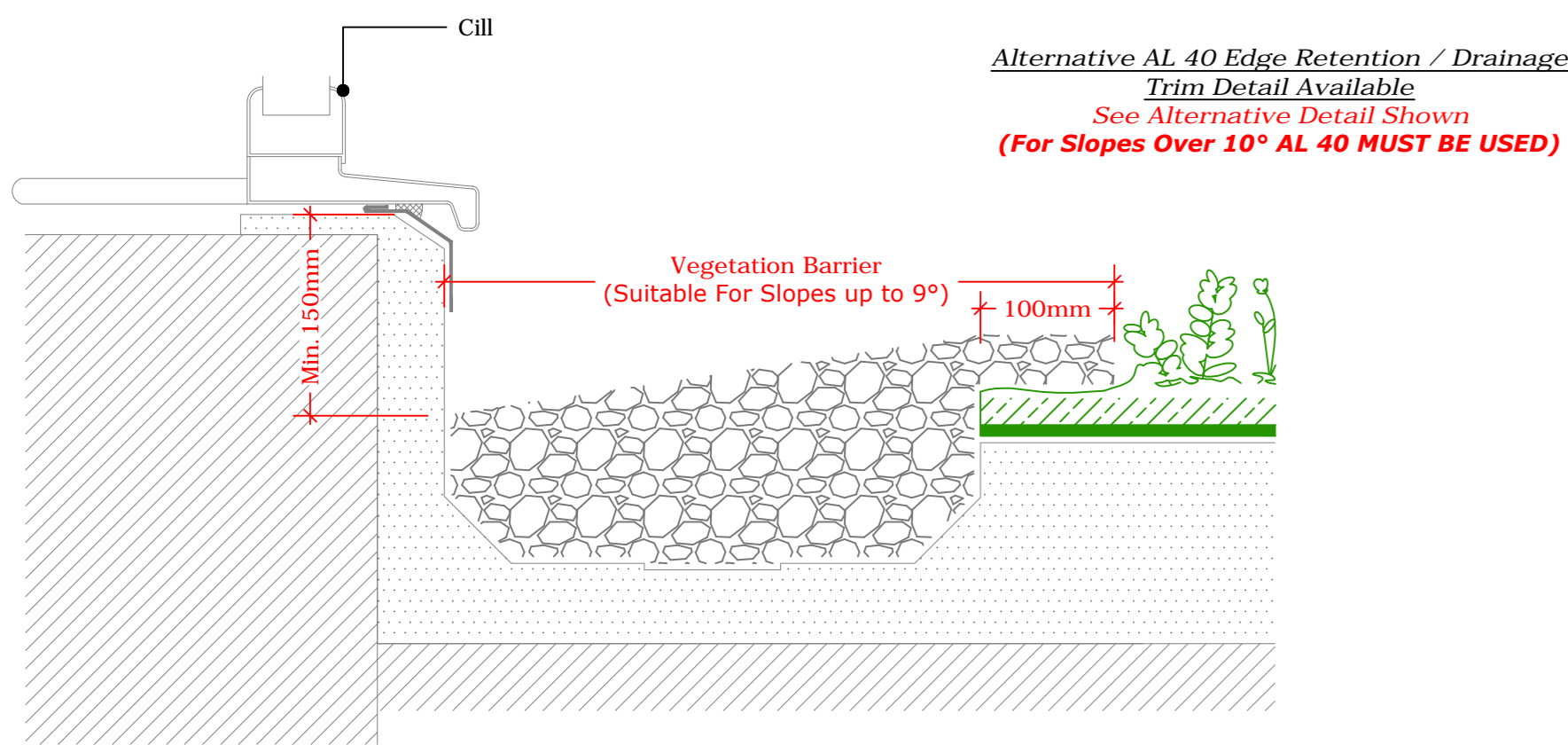
Internal Gutter to Clerestory Window (Drg.No: D0901-00W_3Deg+_206-Ext-XF301_003)
