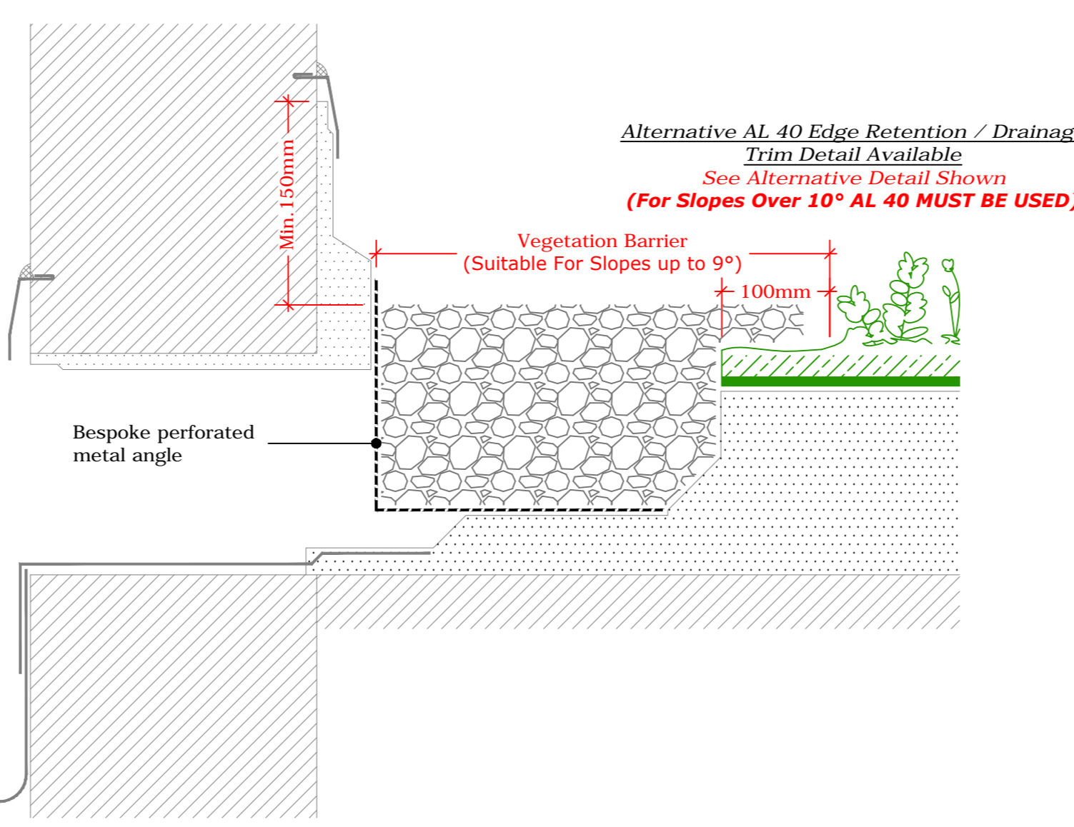
Upstand - Lead Chute (Drg.No: D0901-00W_3Deg+_201-Ext-XF301_002)
