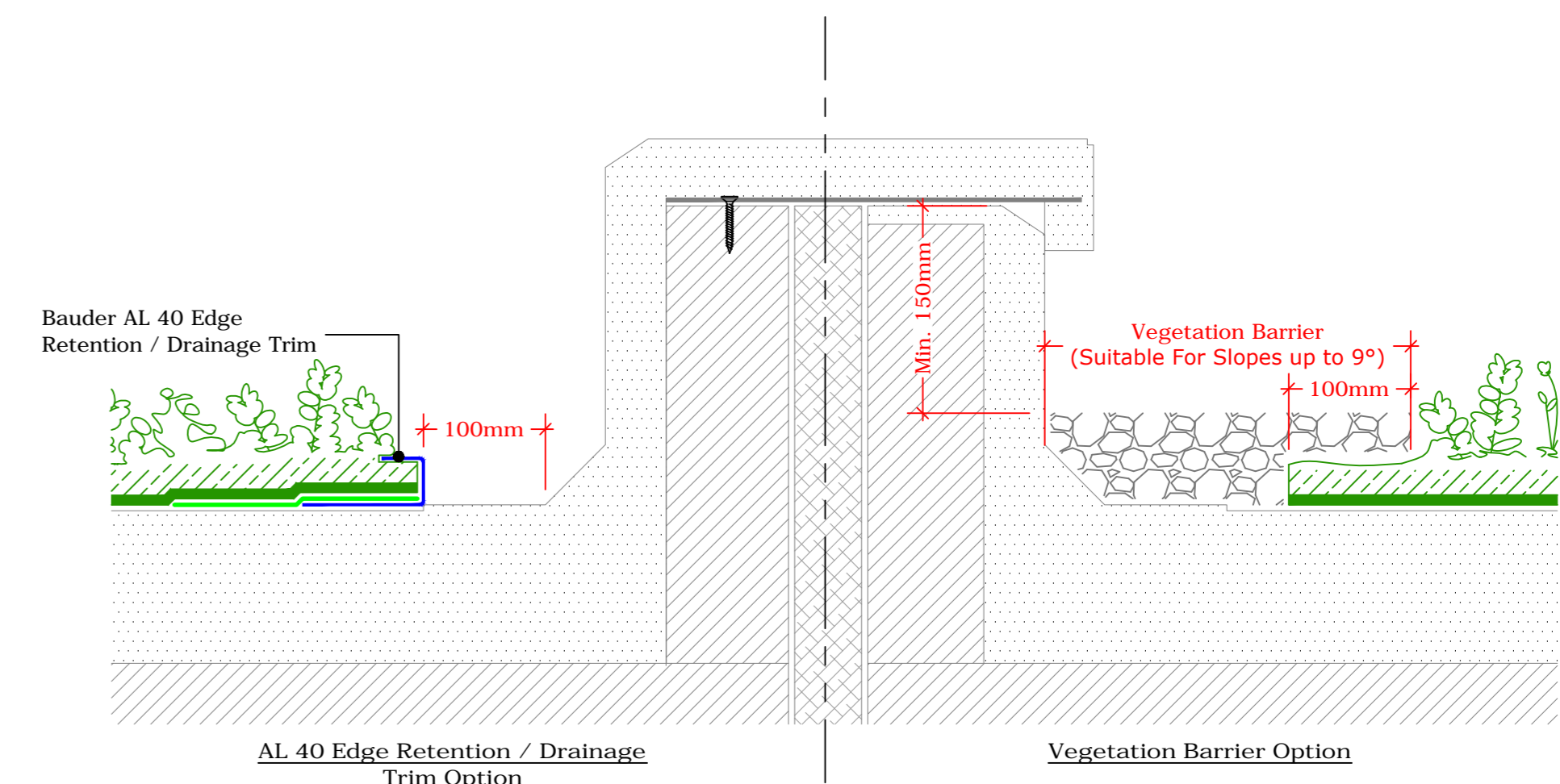
Twin Kerb Expansion Joint (Drg.No: D0901-00W_3Deg+_204-Ext-XF301_001)
