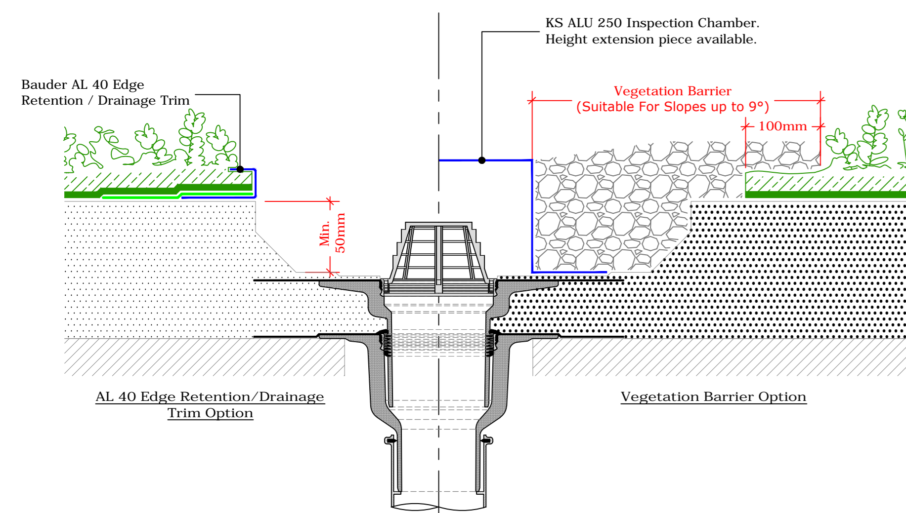
Bauder Outlet - Compact (Drg.No: D0901-00W_3Deg+_008-Ext-XF301_001)
