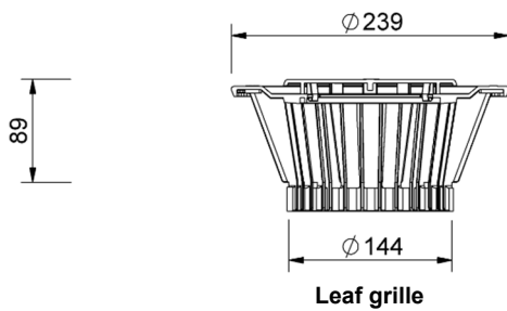
Leaf grille
