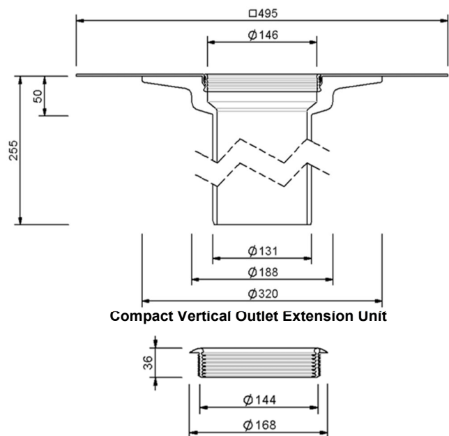
Webbed Insertion Flange
